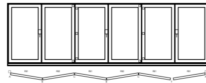
Style 651 5 folding 1 Main
