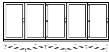
Style 550 5 folding 0 Main
