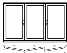
Style 321 2 folding 1 Main
